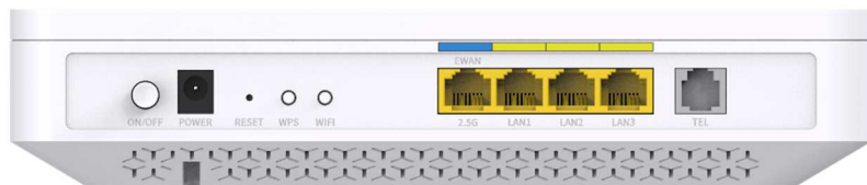
Fig2. Rear Panel
